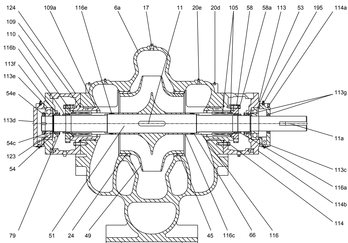
Sectional drawing, optional construction type 11
