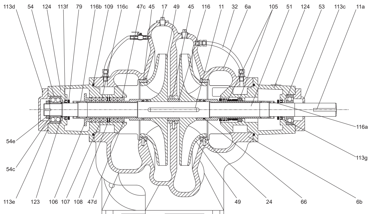
Sectional drawing, standard construction type 14
