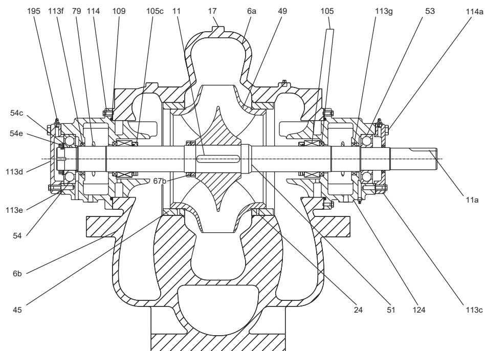
Sectional drawing, standard construction type 1
