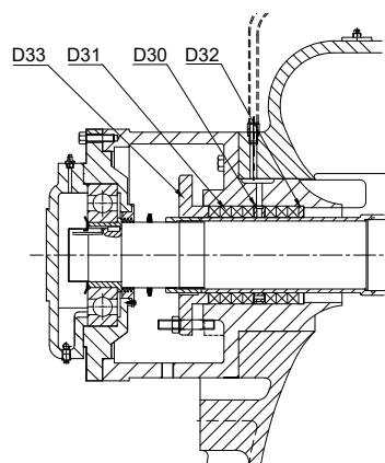
Sectional view of stuffing box
