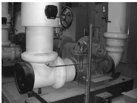
LS pump in a commercial building application
