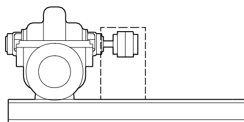
Bare shaft pump with common base frame
