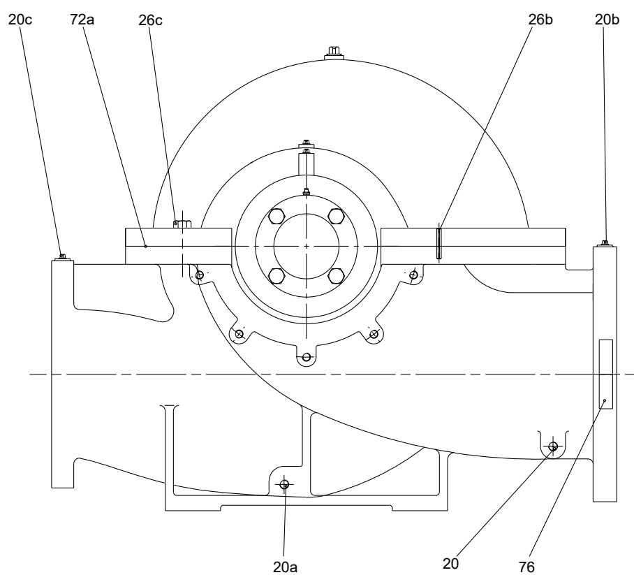
Typical end view, non-drive end
