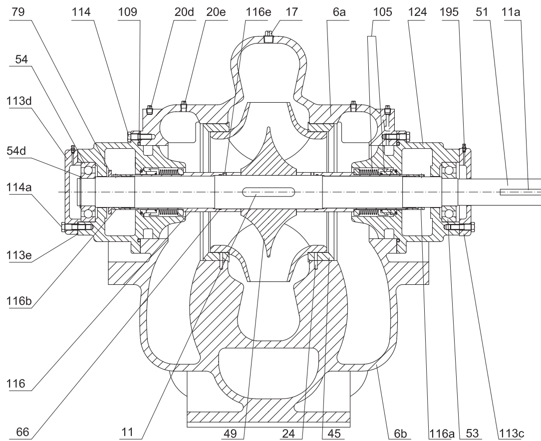
Sectional drawing, optional construction type 10
