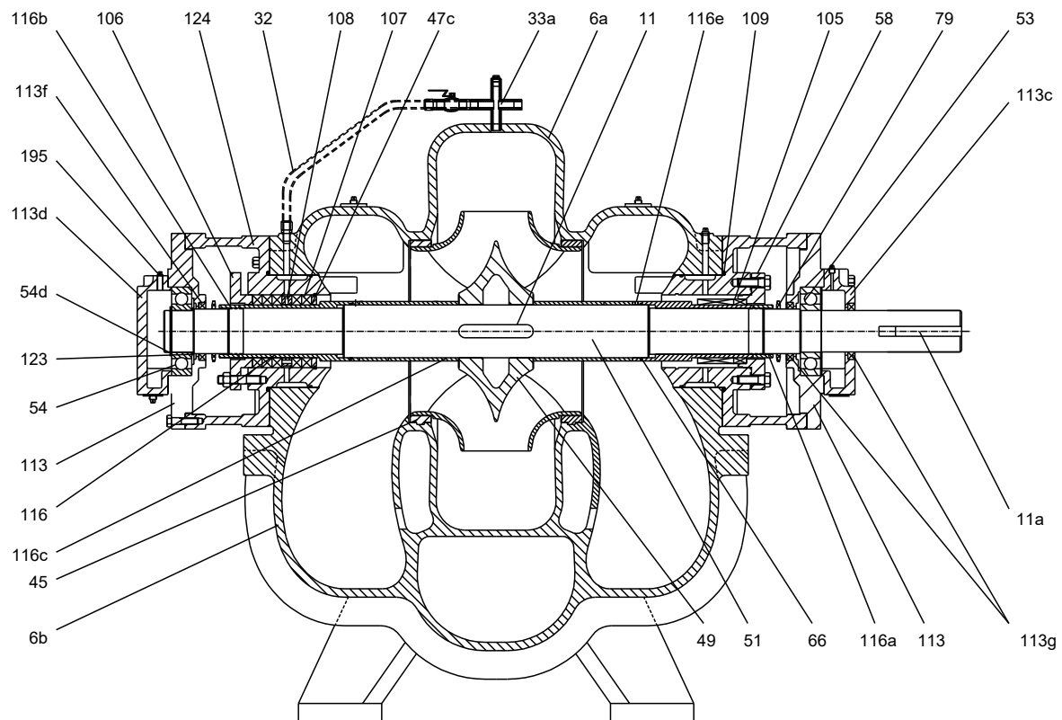
Sectional drawing, optional construction type 13
