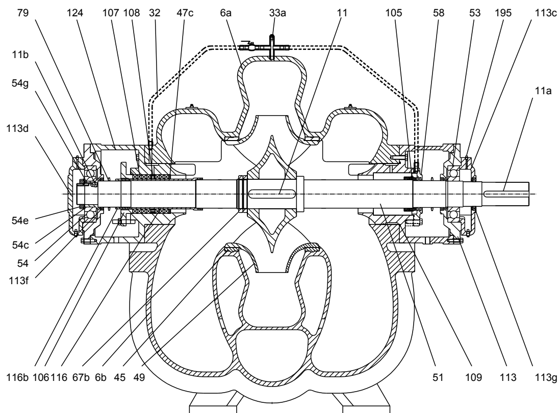
Sectional drawing, standard construction type 5
