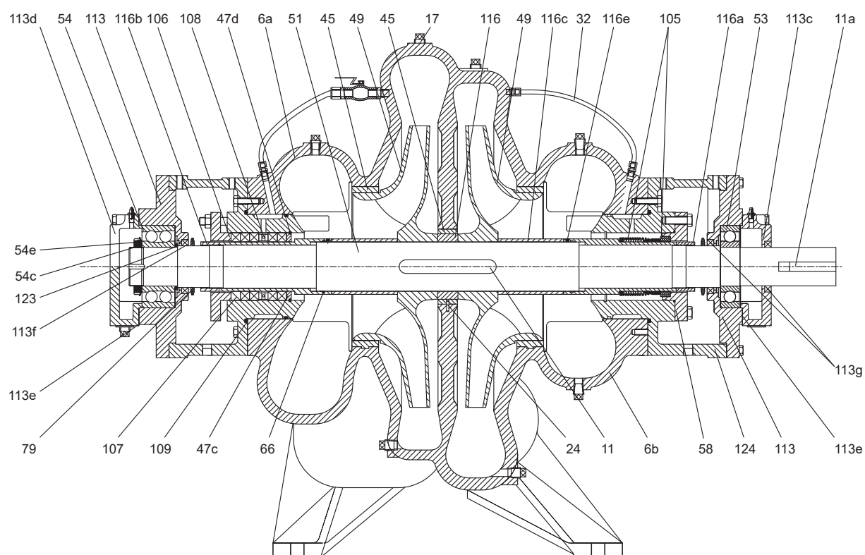
Sectional drawing, standard construction type 15
