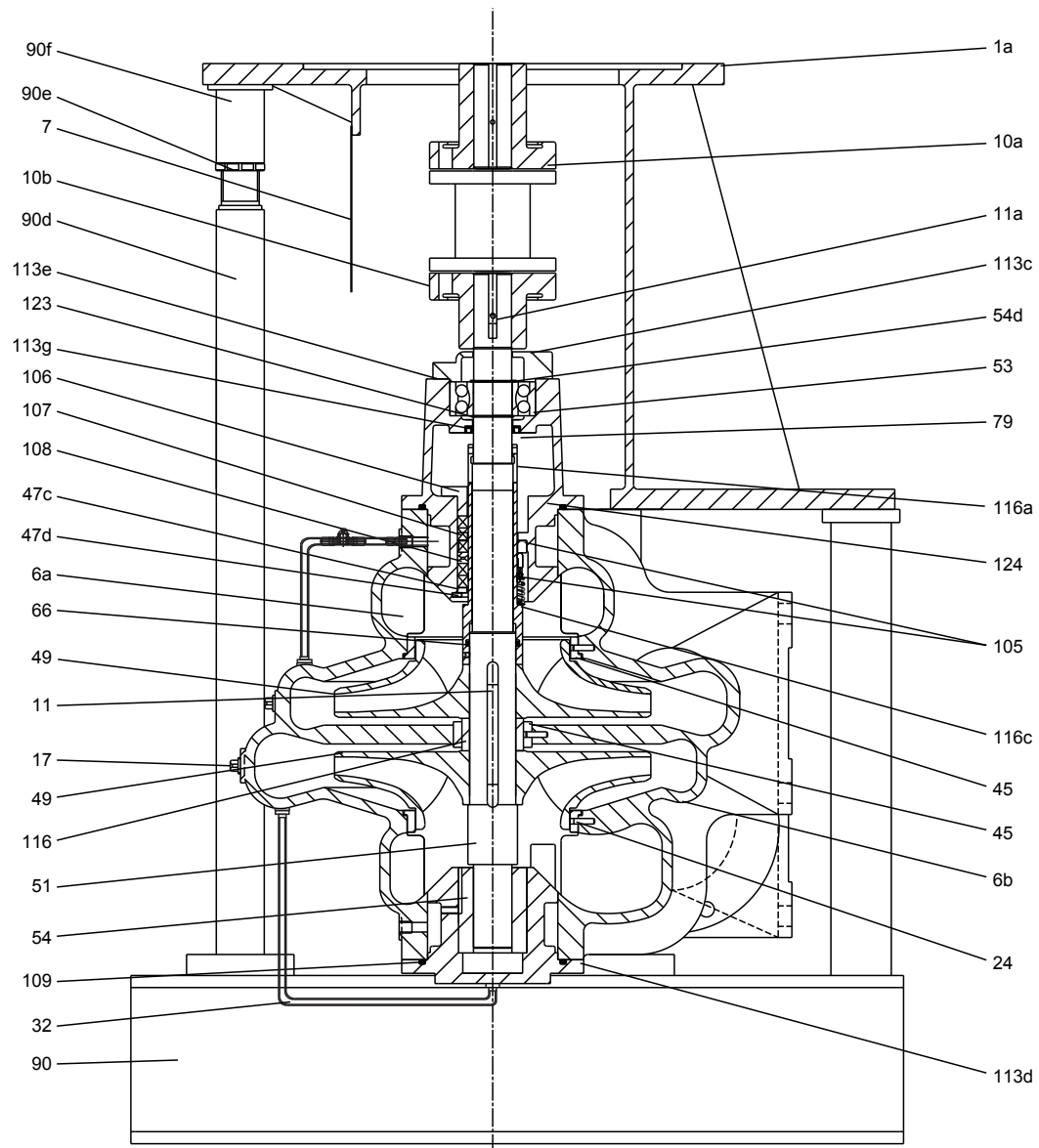
Sectional drawing, standard construction type 16
