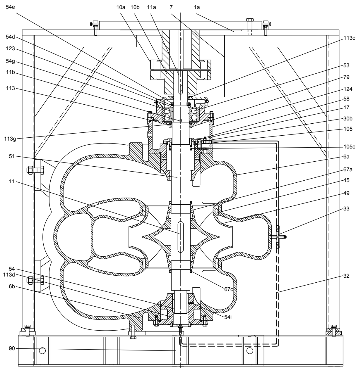
Sectional drawing, standard construction type 9, motor frame size above 400
