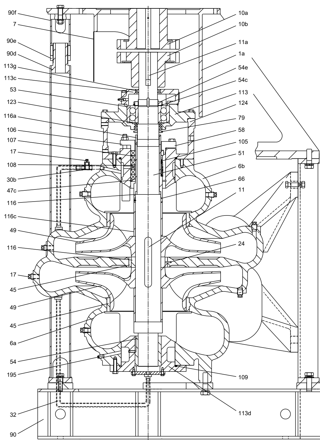
Sectional drawing, standard construction type 17
