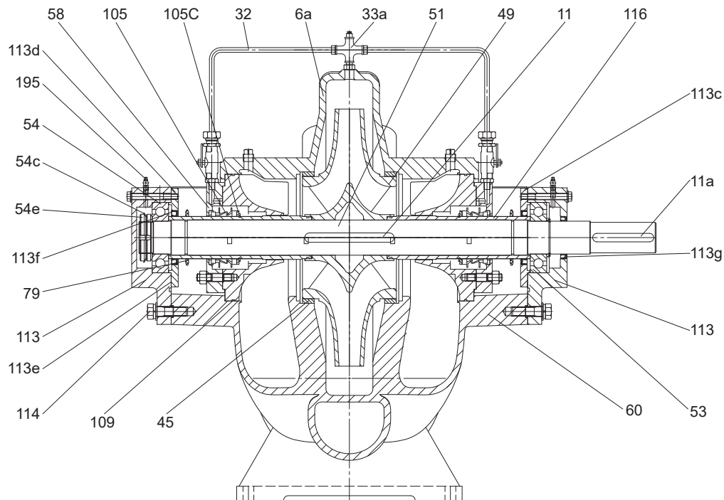
Sectional drawing, optional construction type 4
