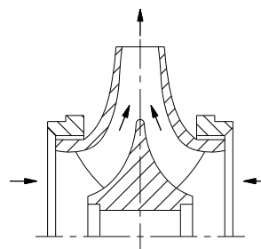
Double-inlet impeller
