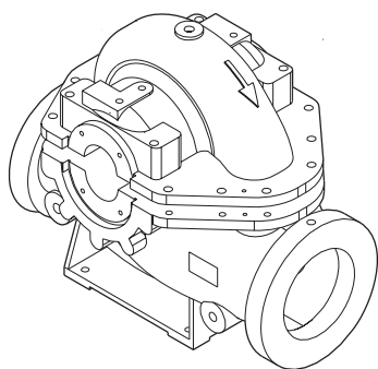
Upper and lower pump casing of LS pump
