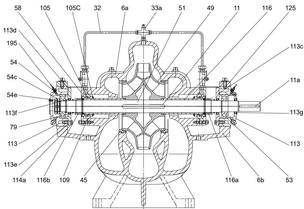
Sectional drawing, standard construction type 3
