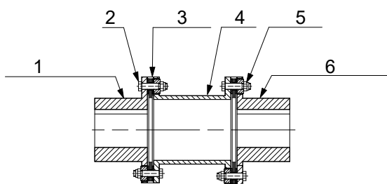
Flexible, laminated spacer coupling construction
