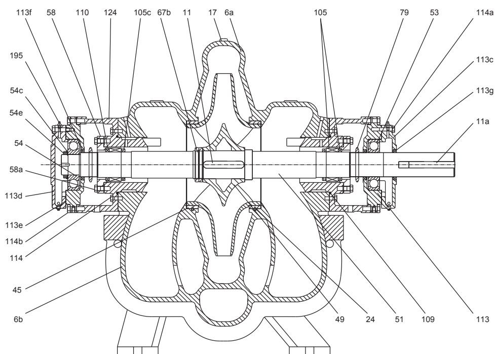
Sectional drawing, standard construction type 2
