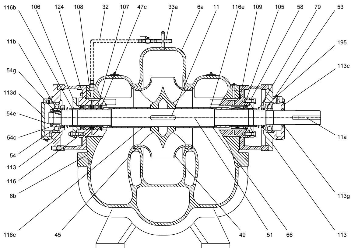
Sectional drawing, optional construction type 12
