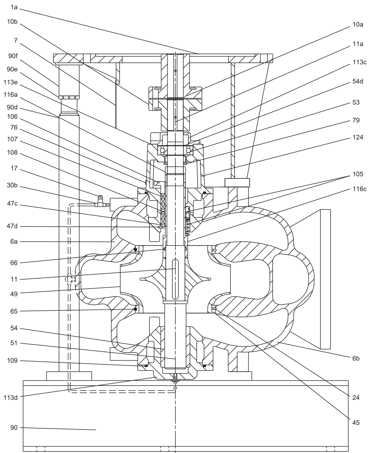
Sectional drawing, standard construction type 7, motor frame size from 280 to 315
